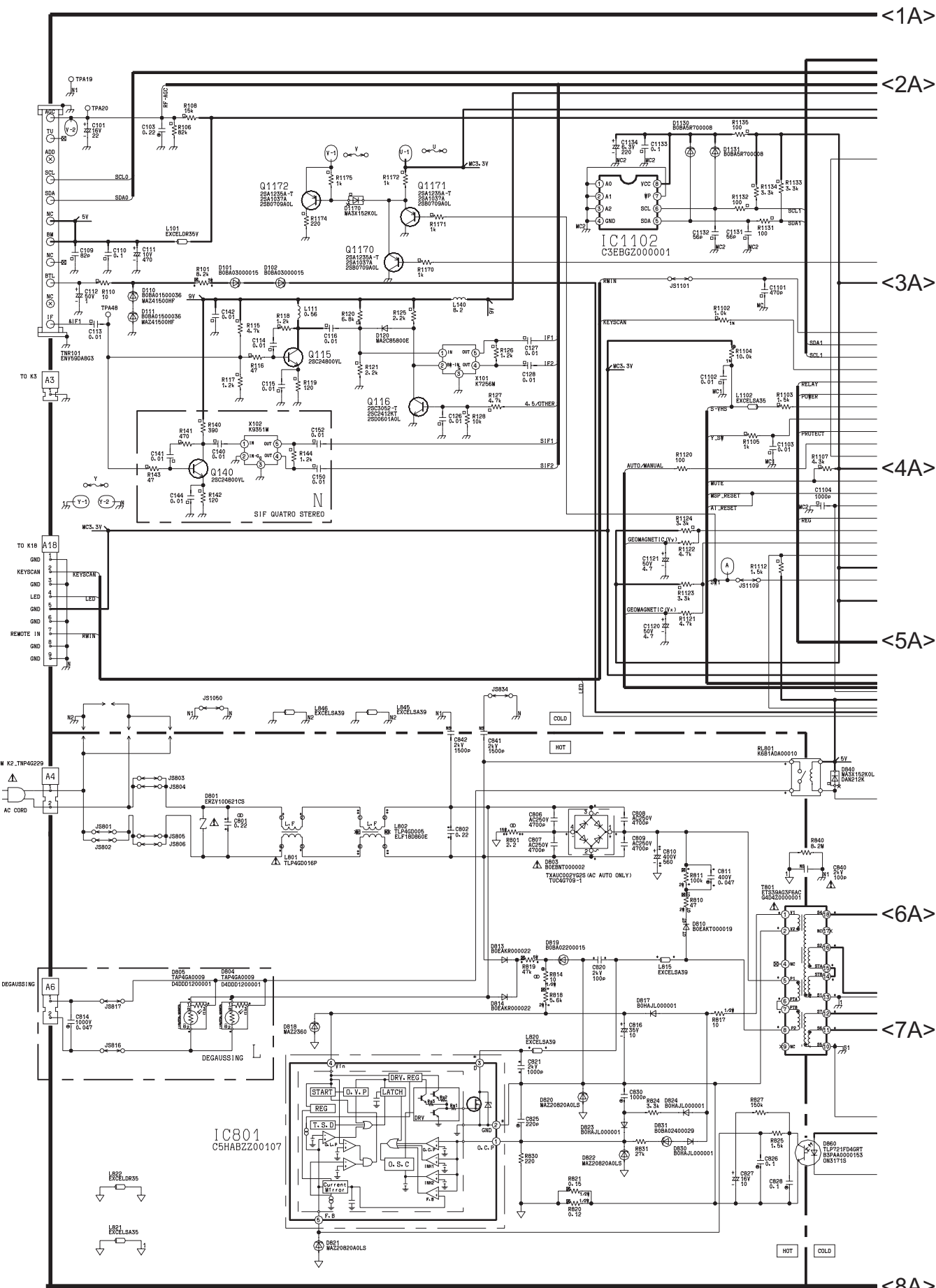
A Board TX-29PS72X Schematic Diagram (1/4)
