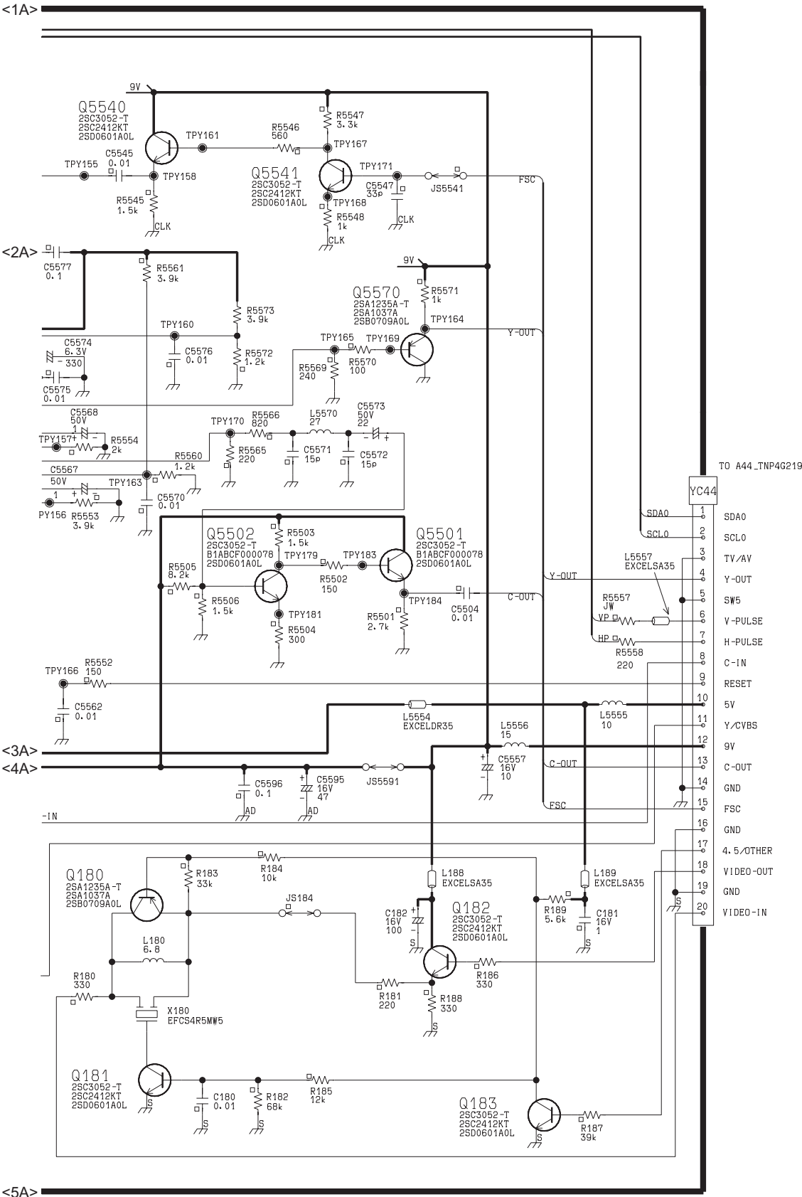
YC Board TX-29PS72X Schematic Diagram (2/2)
