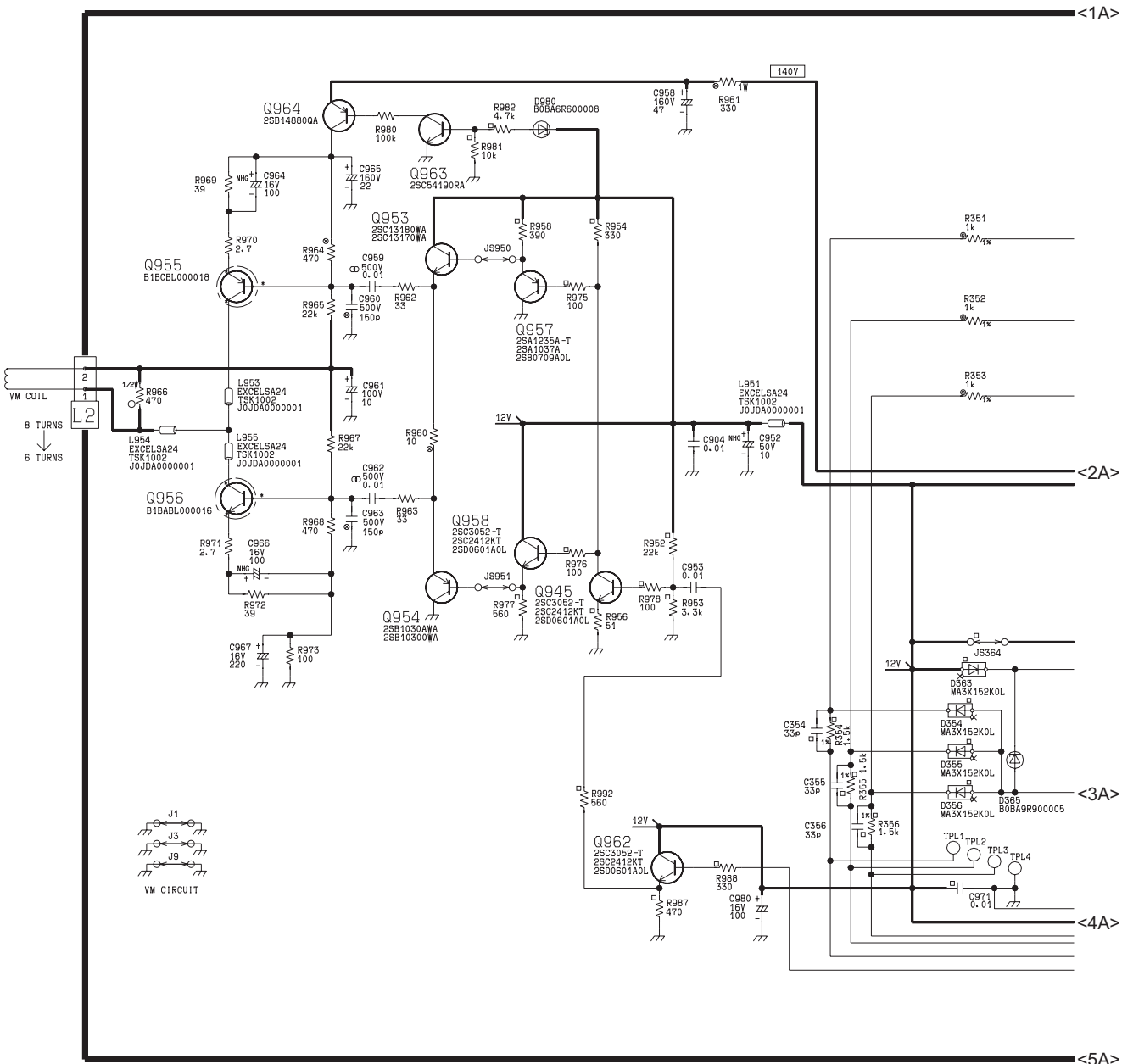
L Board TX-29PS72X Schematic Diagram (1/2)
