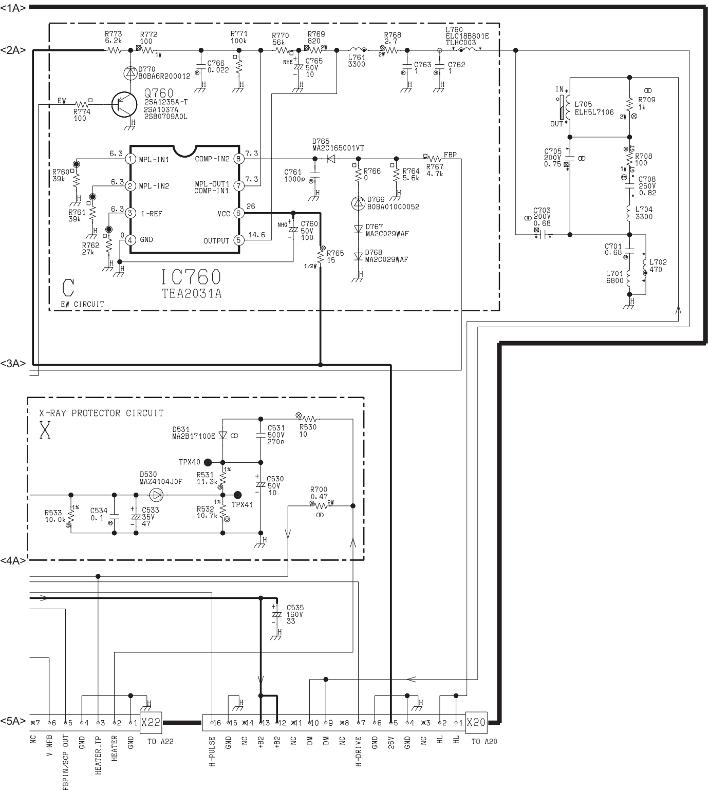
X Board TX-29PS72X Schematic Diagram (2/2)
