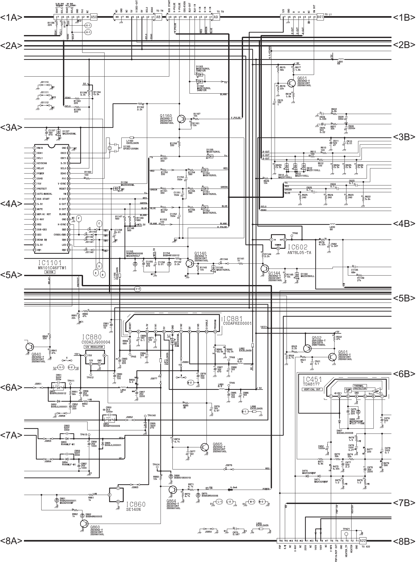
A Board TX-29PS72X Schematic Diagram (2/4)
