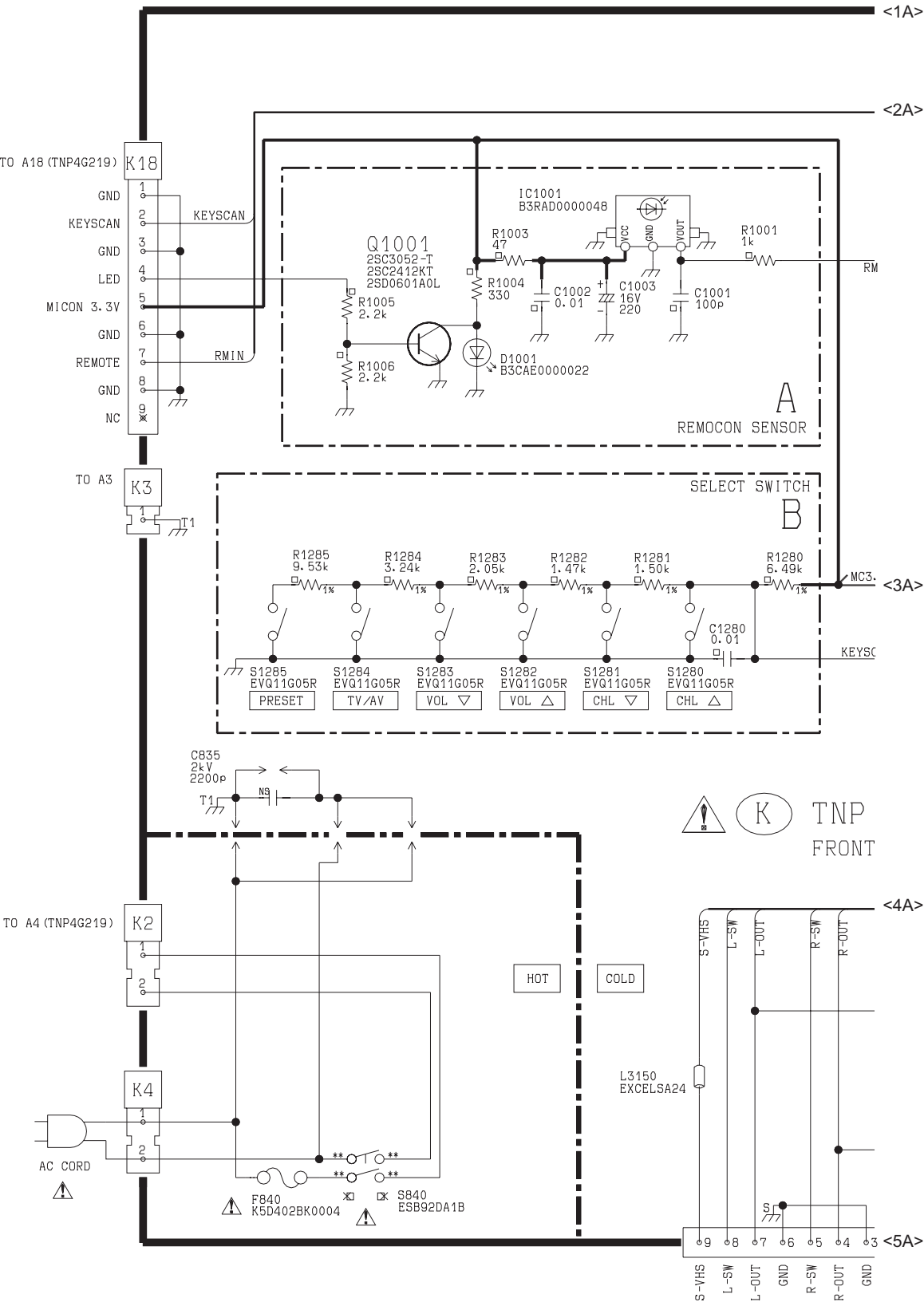
K Board TX-29PS72X Schematic Diagram (1/2)
