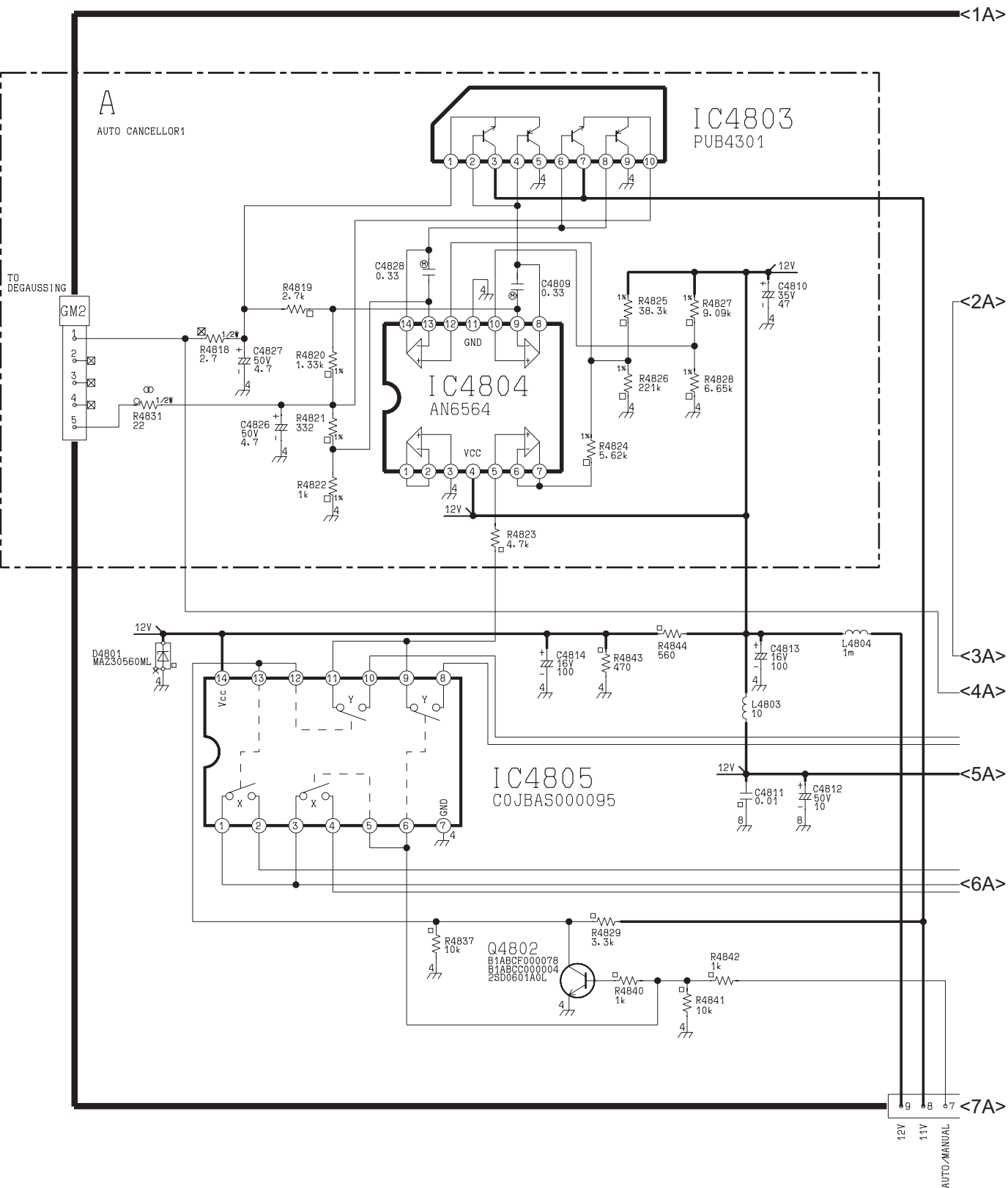
GM Board TX-29PS72X Schematic Diagram (1/2)
