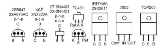
Schematic of 250W ATX power supply with active PFC (reverse engineered by Vladimir Davydov). Annotated by http://www.smpsowersupply.com/
