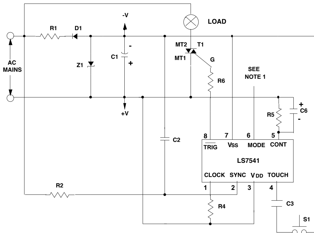
FIGURE 6. PUSHBUTTON APPLICATION SCHEMATIC
