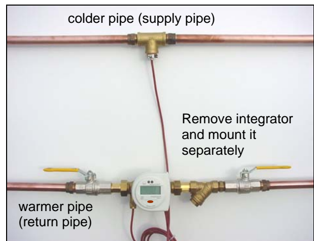
fig. 2: PolluCom EX/S in a cooling plant
