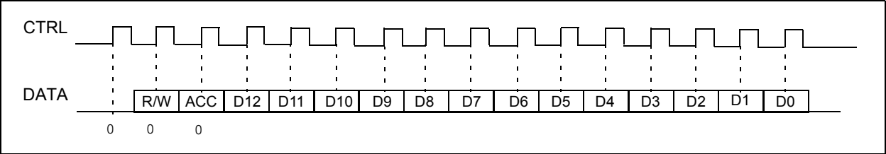
FIGURE 28-3: CONFIGURATION REGISTER 'WRITE'
