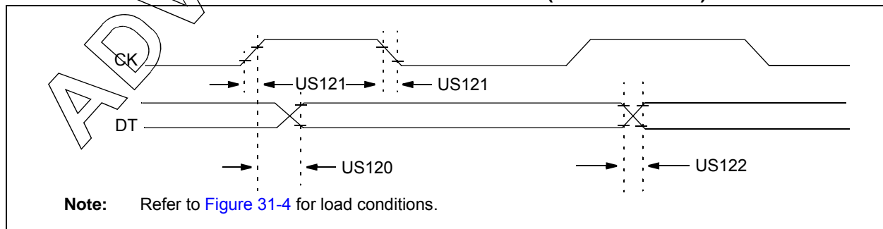
FIGURE 31-13: USART SYNCHRONOUS TRANSMISSION (MASTER/S�AVE) TIMING
