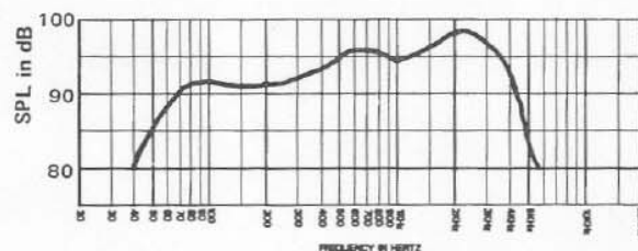
FIGURE 2 - TL606/EVM.15B Frequency Response (Swept 1/3-Octave Band Pink Noise, 4 V at 10 ft on Axis, Half-Space Environment)
