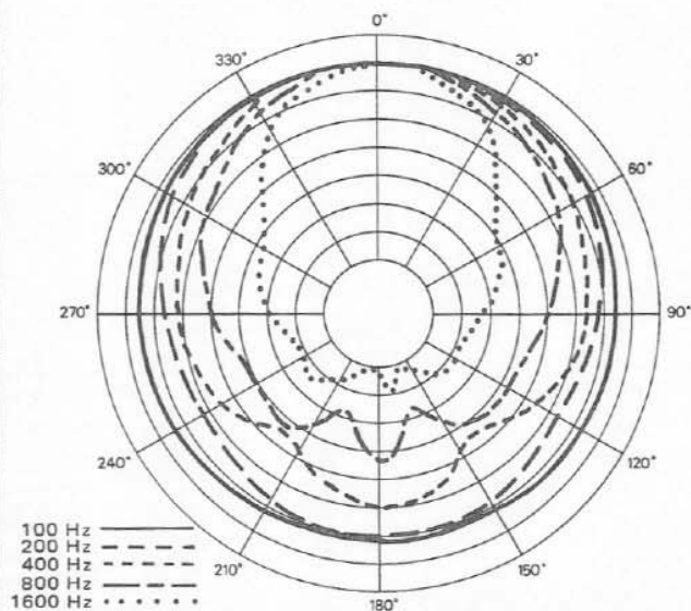
FIGURE 3 - TL606/EVM.15B Polar Response 4 V RMS of Octave Band Limited Pink Noise in Anechoic Environment, 10 ft on axis in Horizontal Plane (5 dB per Division)
