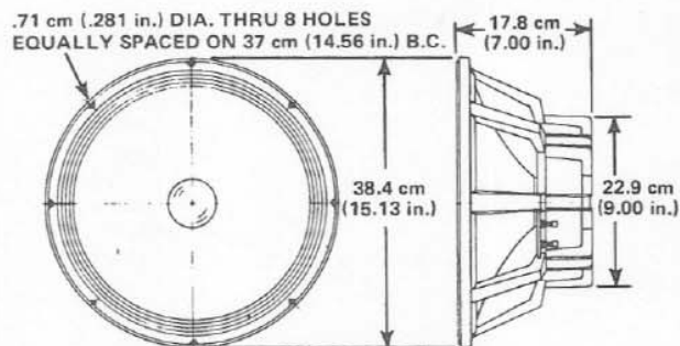
FIGURE 1 - Dimensions
