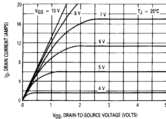
Figure 2. On-Region Characteristics
