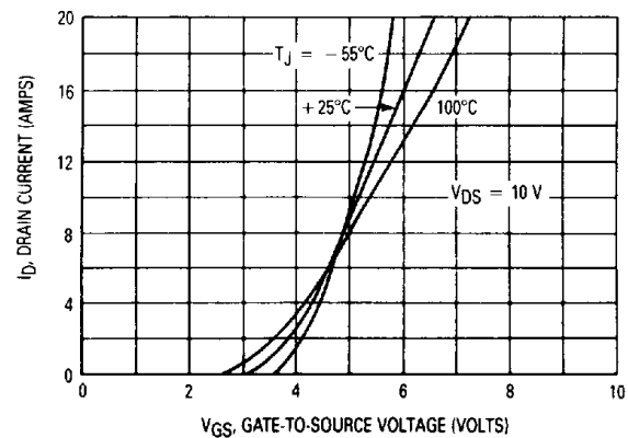
Figure 4. Transfer Characteristics
