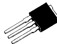
CASE 369-06 TO-251 MTD10N05E1
