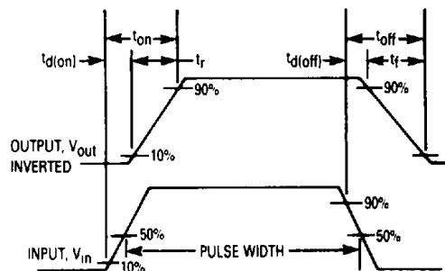
Figure 19. Switching Waveforms
