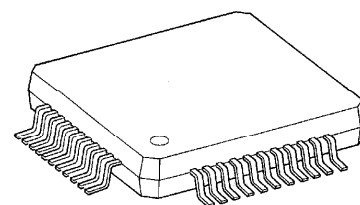
QFP44-P-1414-0.80D
