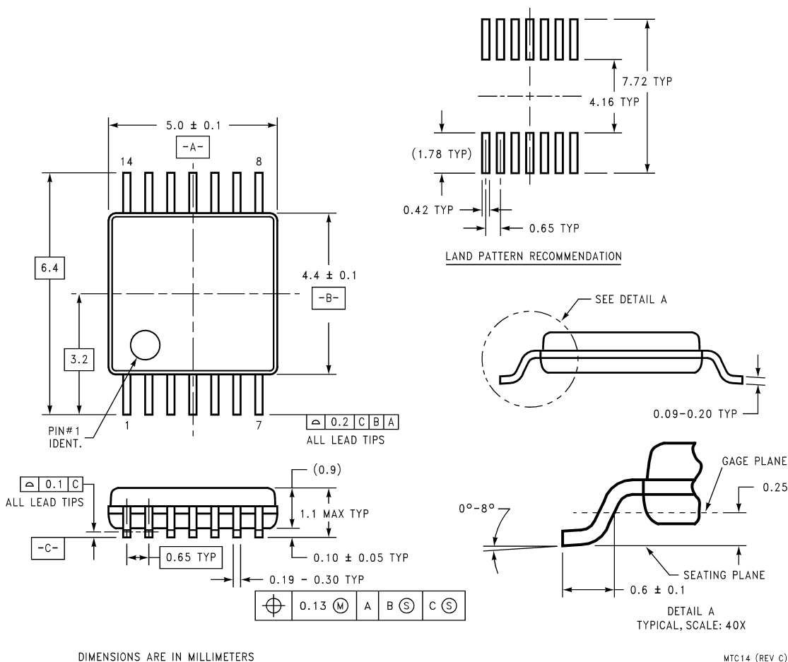
TSSOP-14 Pin Package (MTC) For Ordering, Refer to Ordering Information Table NS Package Number MTC14
