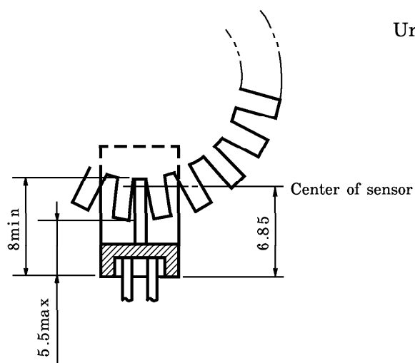
Cross section between A and A'
