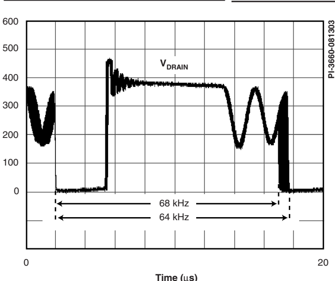
Figure 4. Frequency Jitter.
