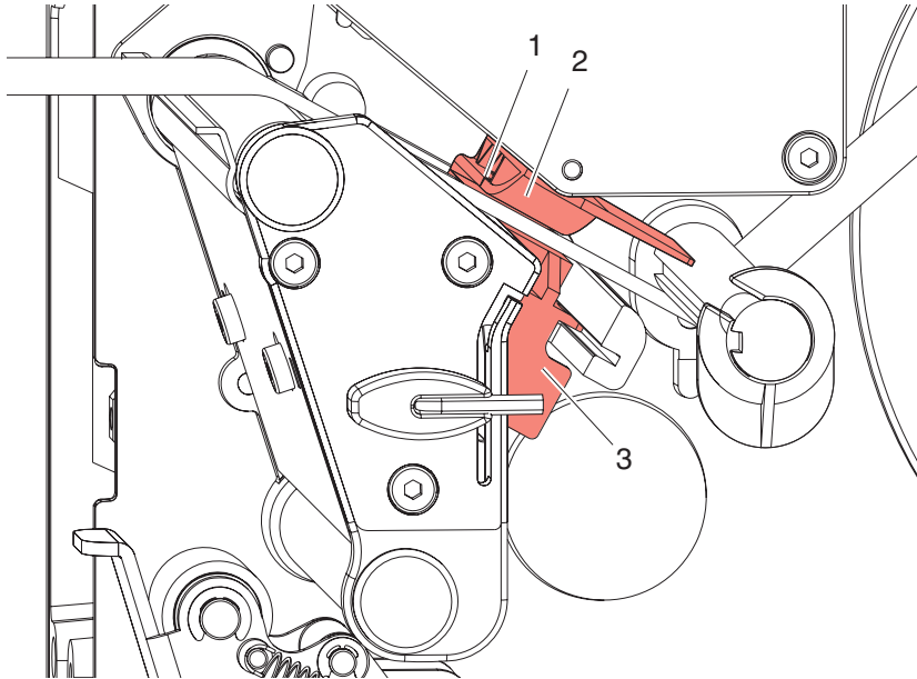
Fig. 6: Setting the label sensor
