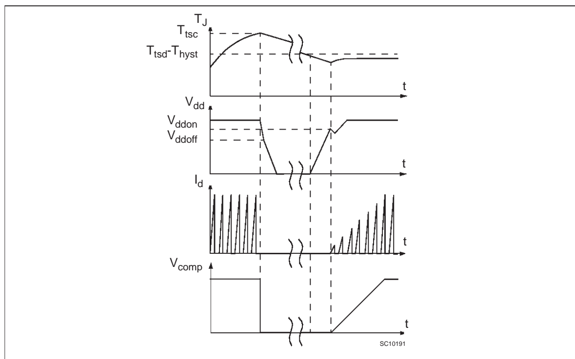
Figure 8: Overtemperature Protection
