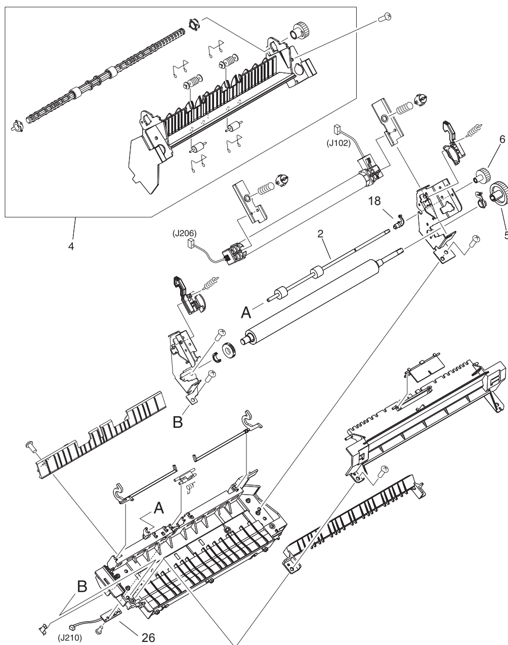
Figure 94. Fuser assembly
