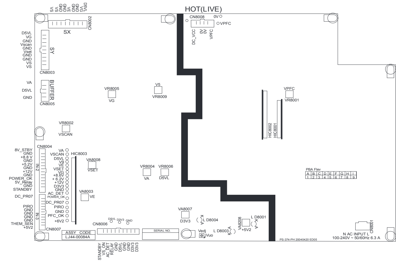
Figure 6-9 PSU layout
