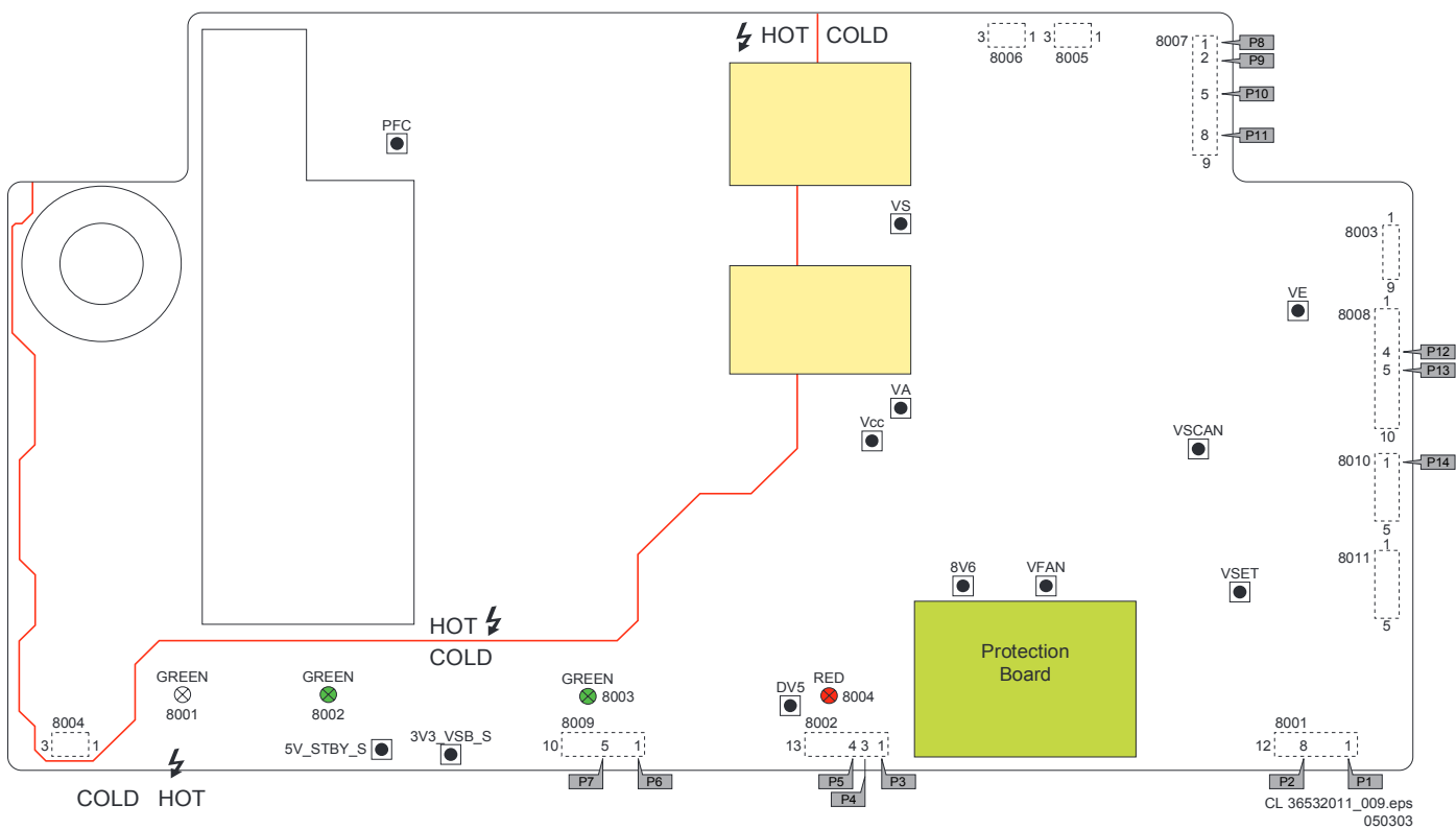
Figure 6-10 PSU layout
