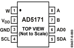
Figure 4. SOT-23-8
