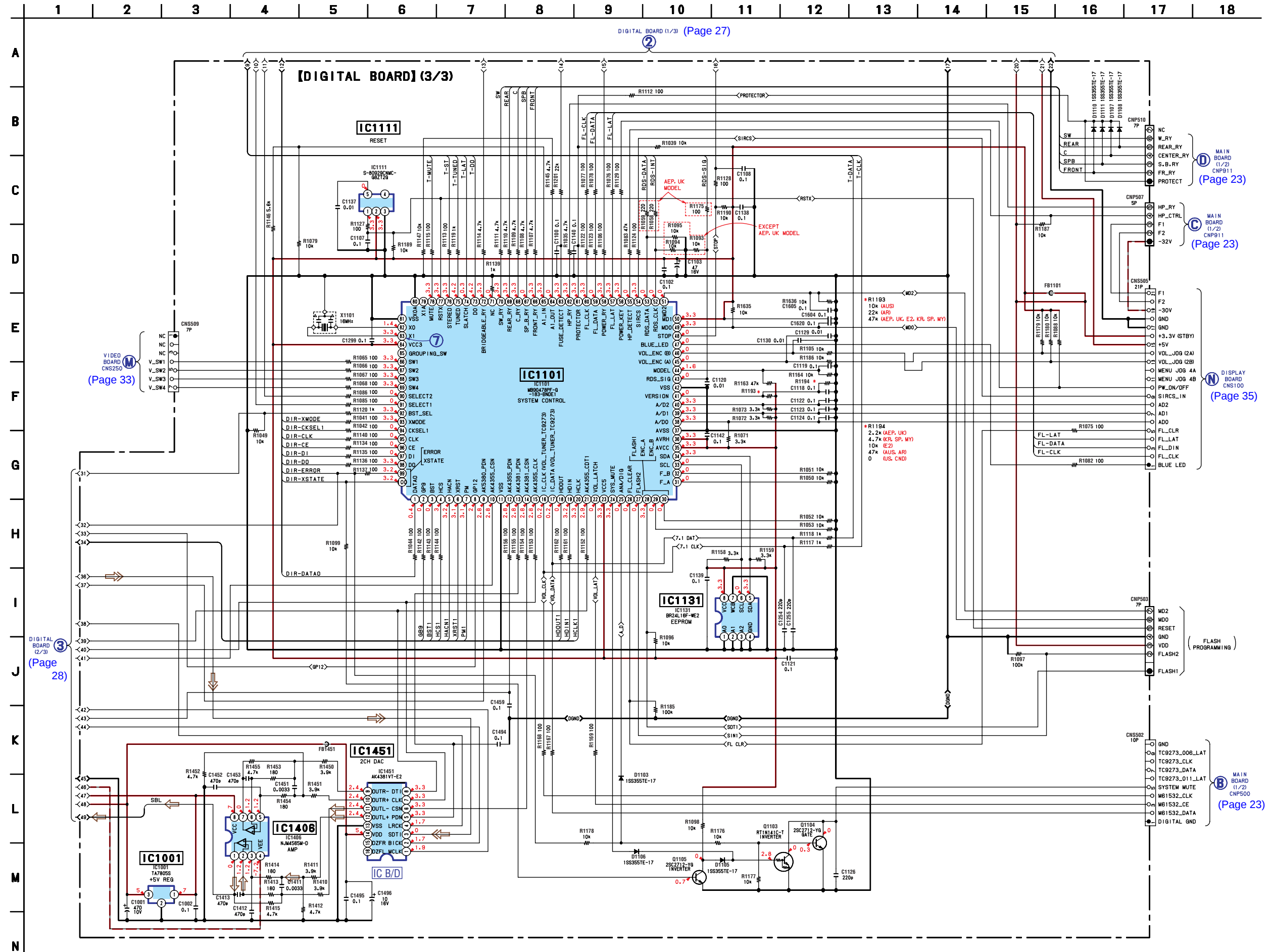
4-15. SCHEMATIC DIAGRAM — DIGITAL SECTION (3/3) — • Refer to page 21 for Common Note on Schematic Diagram and Waveforms and page 38 for IC Block Diagrams.
