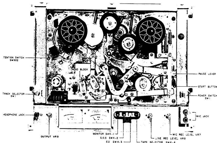
Fig. 2 Front View (GX-4000D)
