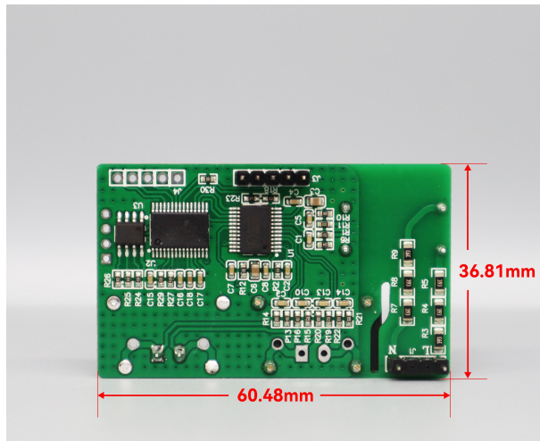
Fig. 2.1 outline and dimension diagram (unit: mm)
