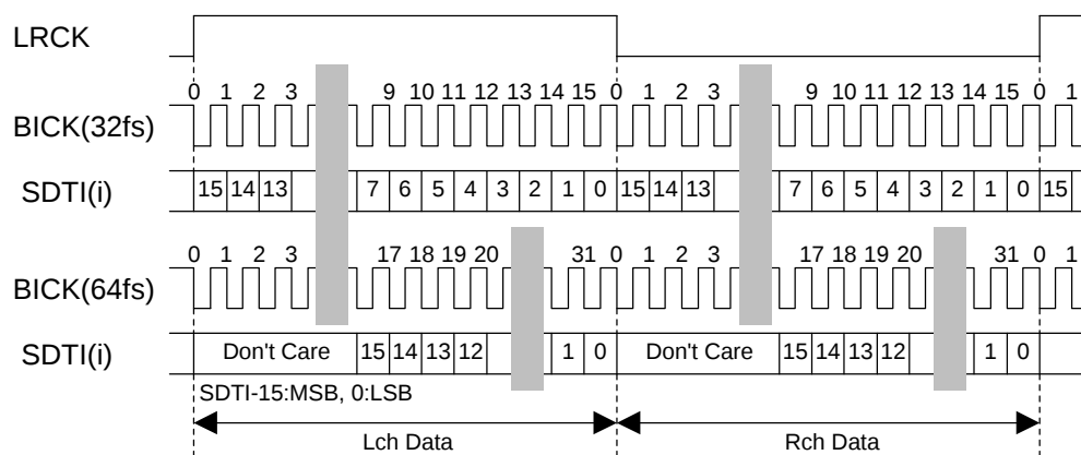
Figure 1. Mode 0 Timing
