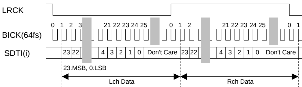
Figure 4. Mode 3 Timing
