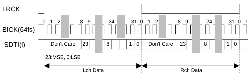
Figure 2. Mode 1 Timing
