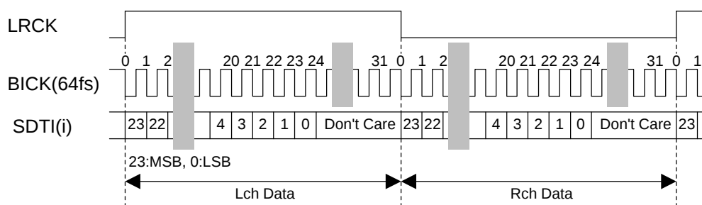
Figure 3. Mode 2 Timing
