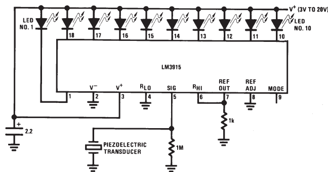
Vibration Meter
